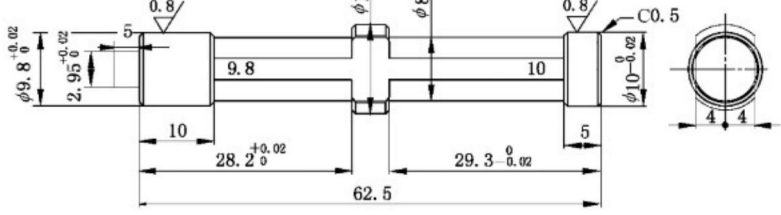
CC1/A+/A-/S+/S- 通止规 9.8
